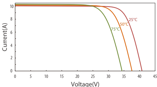
IV Curves of JT325SHh at different Temp
