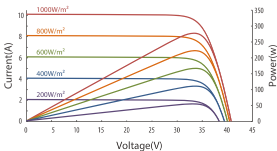
IV Curves of JT325SHh at different irradiances
